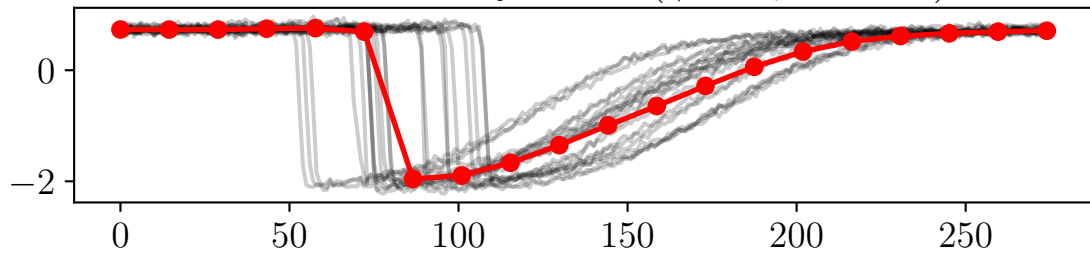
Soft-DTW barycenter ( \gamma = 1, N = 20 )
