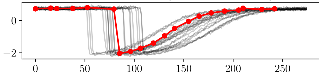
FGW barycenter ( \alpha = 10^{-6}, N = 20 )
