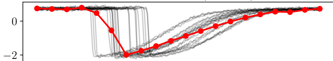
DBA barycenter ( N = 20 )
