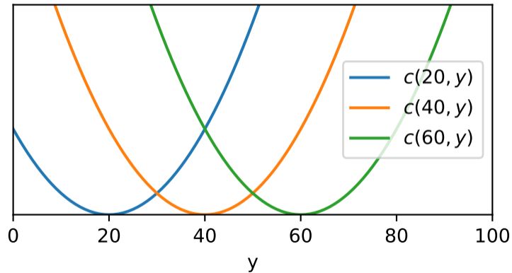
Quadratic cost c(x, y) = |x - y|^2
